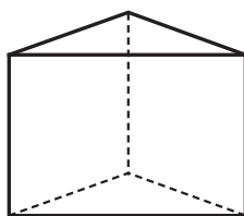
Prisma triangular
