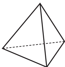
Tetraedro
